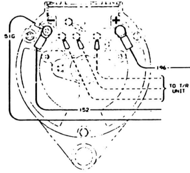
VIEW A A TEST-LAMP SCALE 1:1
