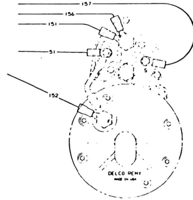
VIEW D STARTER MOTOR SCALE 1:1
